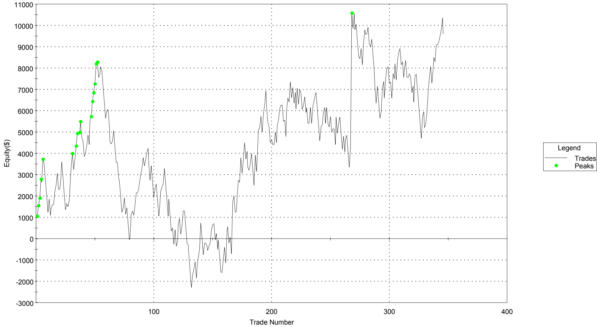
Equity Curve Line - GCZ08 1 min(07/31/08 08:31 - 11/04/08 15:14)
